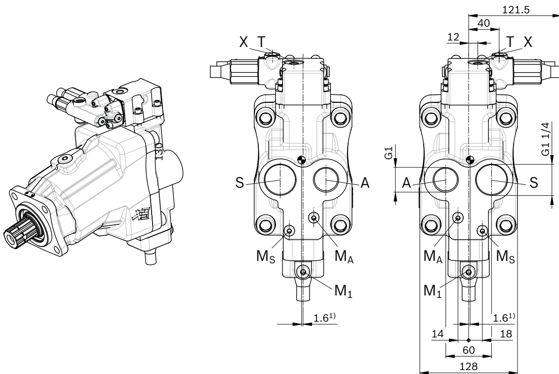
View Y Clockwise rotation
